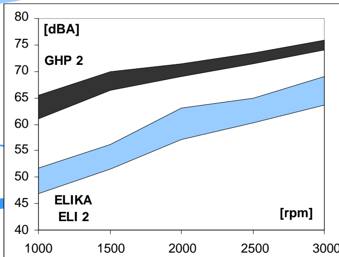
Noise pump comparison [dBA] Marzocchi GHP2 – ELIKA ELI 2, same displacement 17.8 cm 3 /rev.
