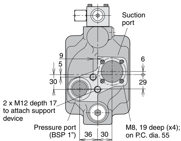
View A-A L.H. rotating pump
