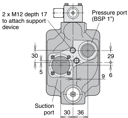
View A-A R.H. rotating pump
