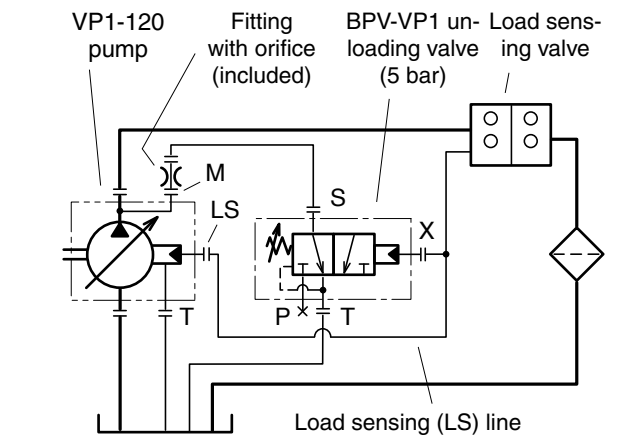
BPV-VP1 installation schematic with VP1-120 pump.
