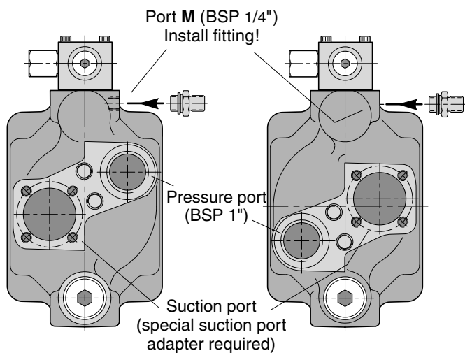
Left hand rotating pump
