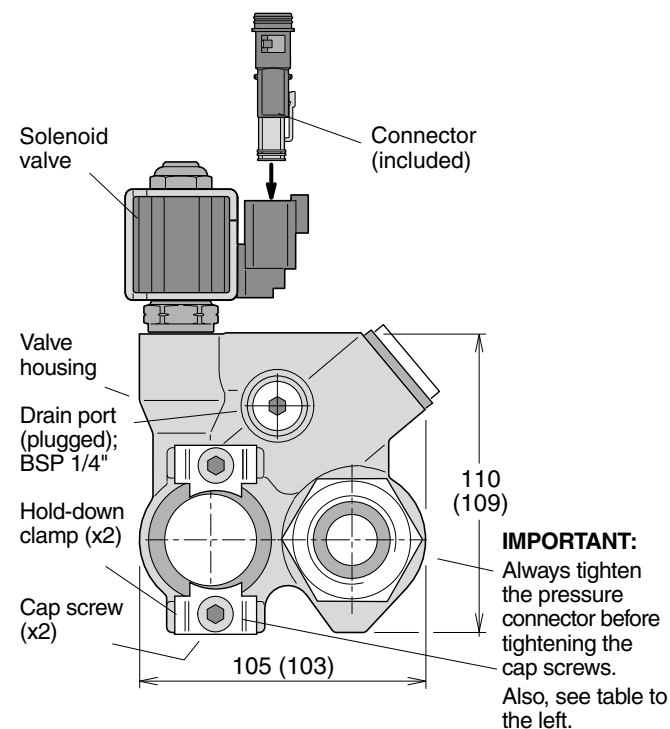
Bypass valve installation and cross section.
